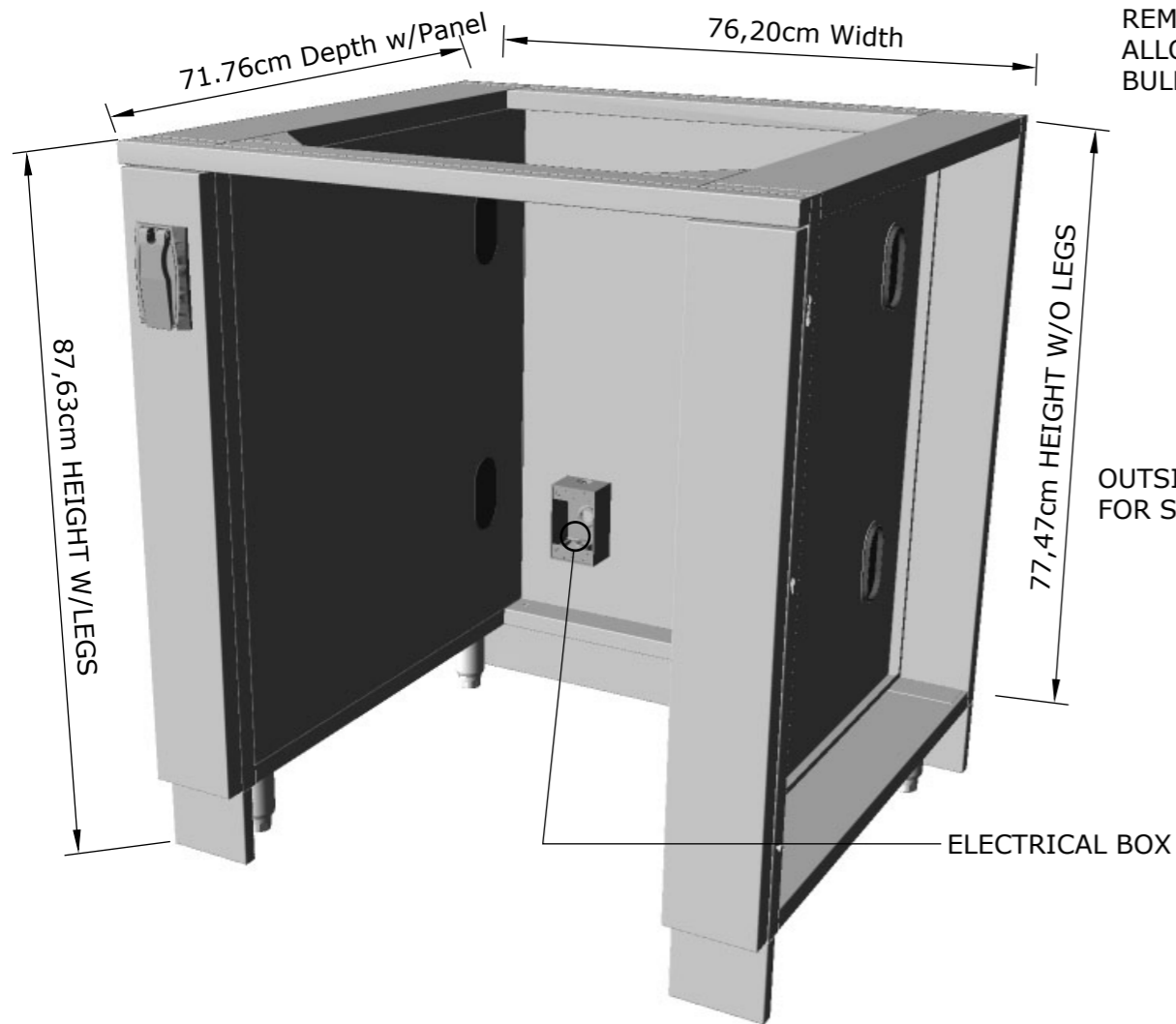
ISO VIEW
